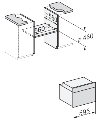
H2840B, H7x4xB/BP/BPX, Skizze
